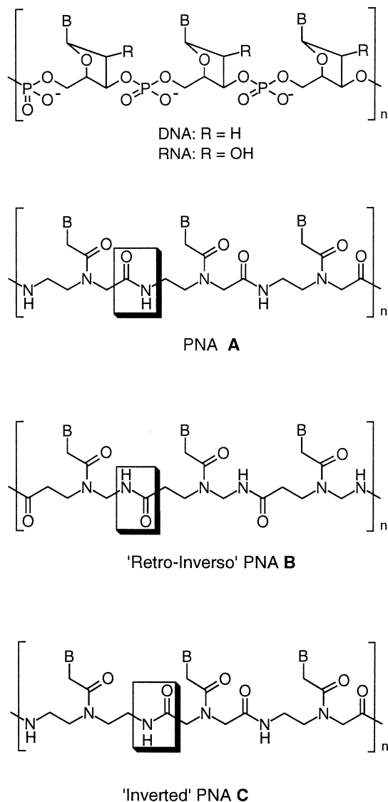
Scheme 1. Upper, peptide nucleic acid (PNA A) with the original N -(2-aminoethyl) glycine backbone; middle, 'retro-inverso' PNA B with the N -(aminomethyl) \beta -alanine backbone; and lower, 'inverted' PNA C. Note the different positioning of polar groups on the backbone, while the number of bonds along the backbone between the nucleobases is kept constant. B = nucleobase.
